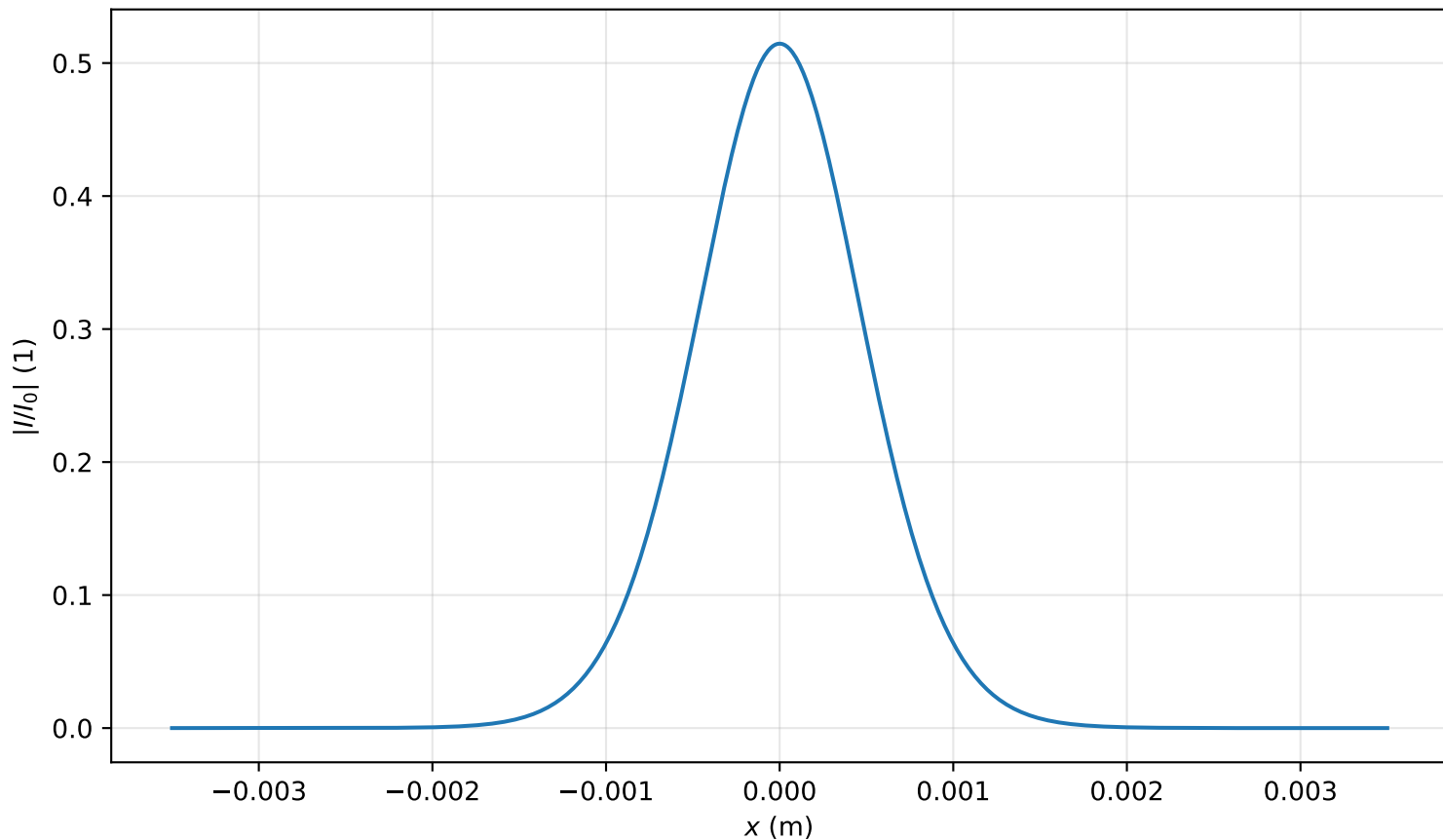
Intensity profile I(x, y = 0, z = 2.548m)/I_0 , P_{in}=0.3P_{cr} , artificial time
